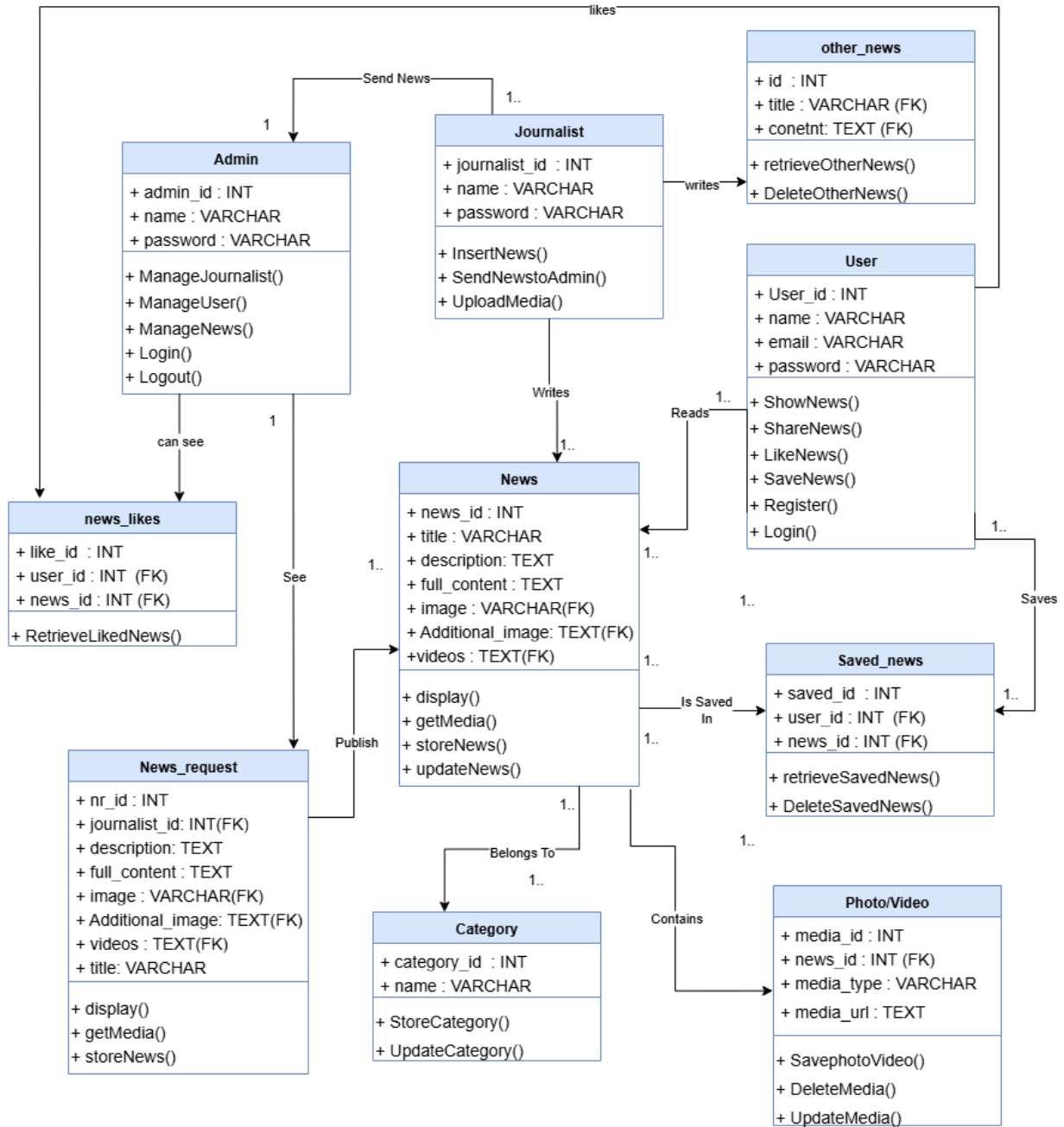
fig. 5: Class Diagram
