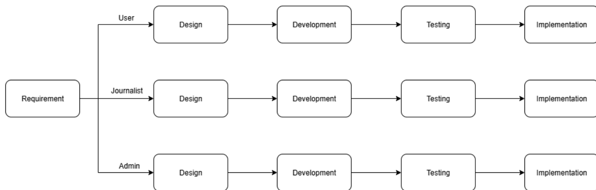
fig. 2: Process Model
